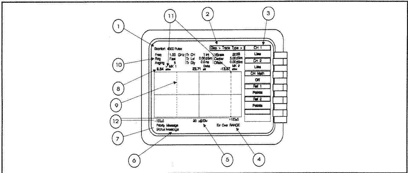
Figure 3-3. Monitor Display
