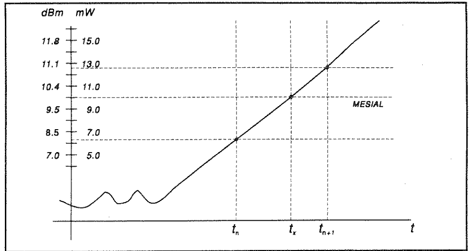
Figure 6-6. Time Interpolation
