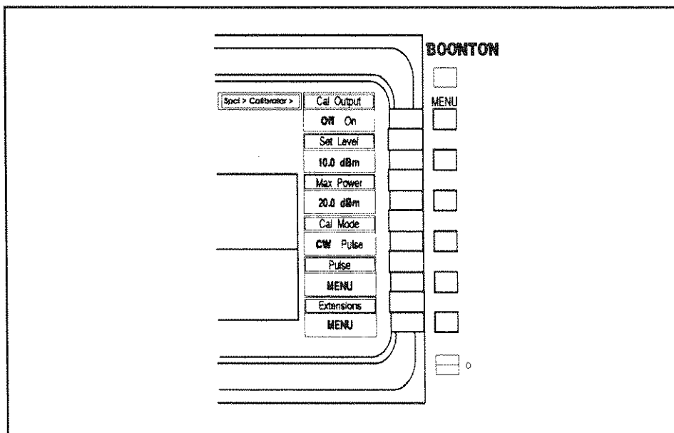
Figure 4-34. Spcl > Calibrator > Menu
