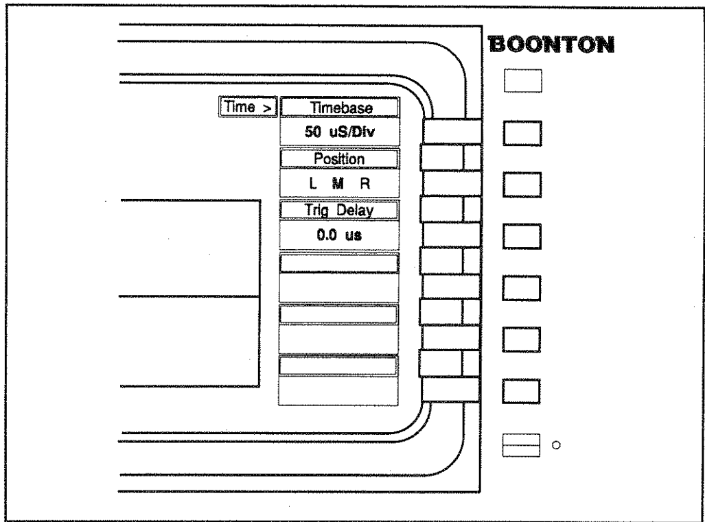
Figure 3-7. Time > Menu
