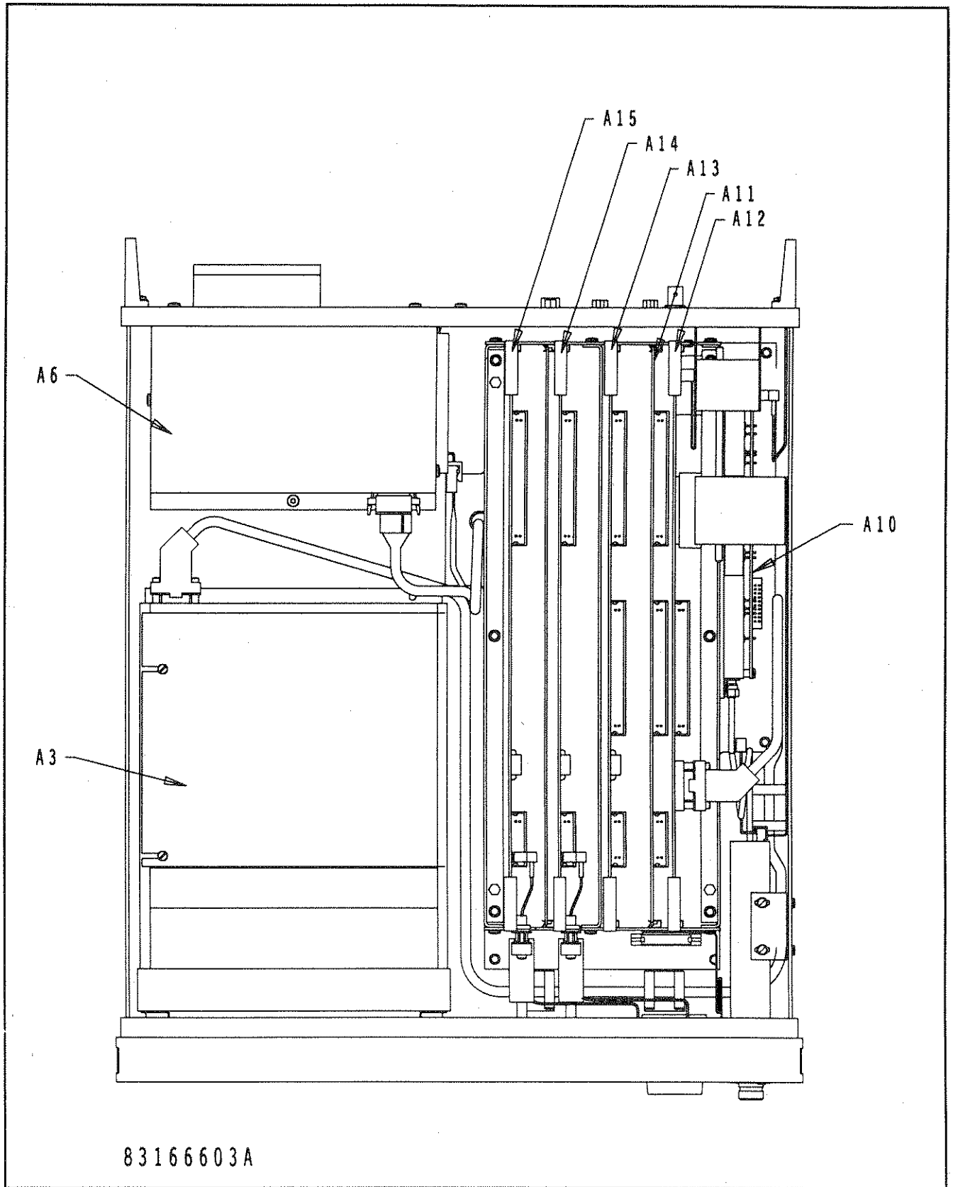
Figure 7-3. Top View of Model 4500 - Cover Removed
