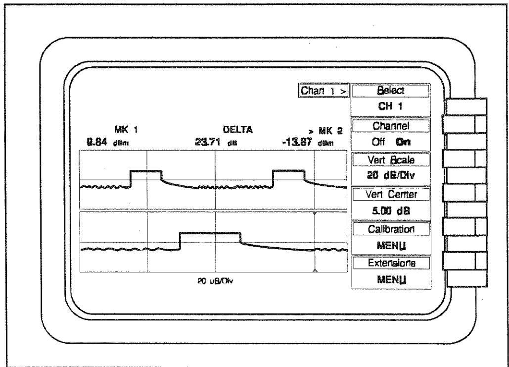
Figure 3-10. Split-Screen Display
