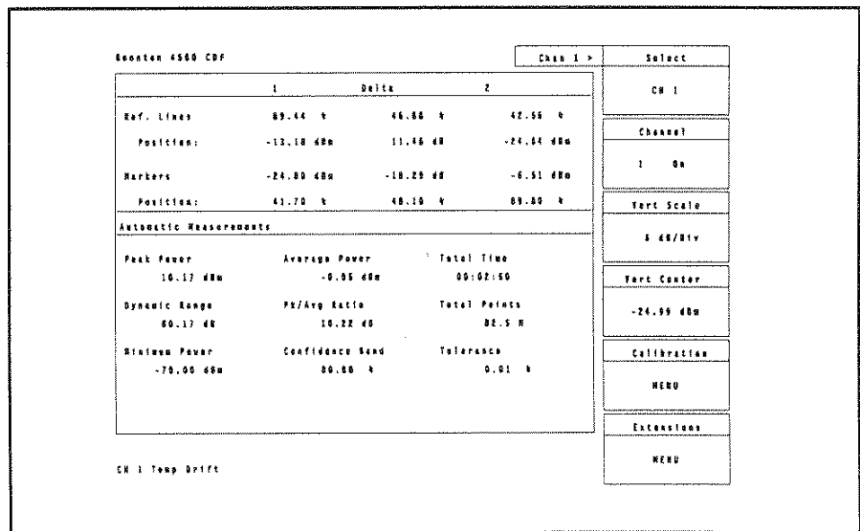
Figure 4-44. Text Mode Display (when in Stat \odot mode)
