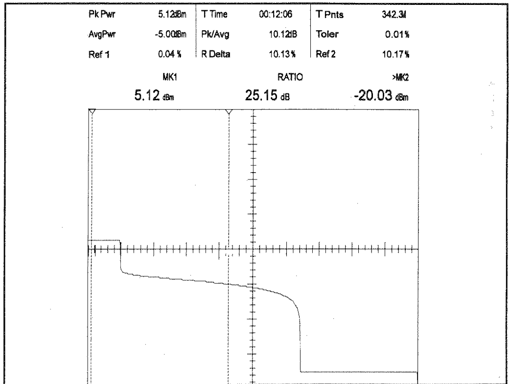
Figure 3-14. 1-CDF Display
