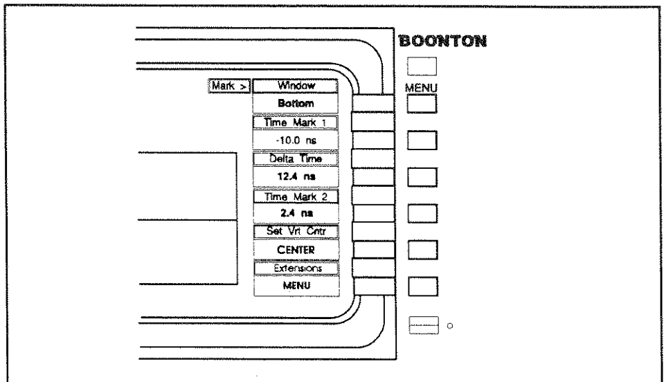
Figure 4-5. Mark > Menu
