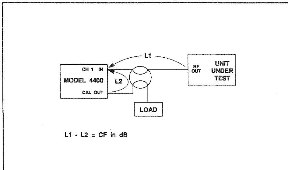
Figure 4-15. Illustration of Measurement (L1) and Calibration (L2) Paths
