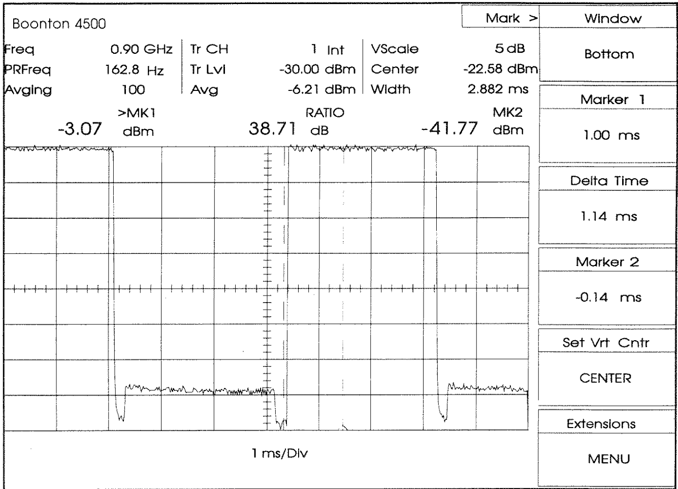
Figure B-3. Sample Output Plot
