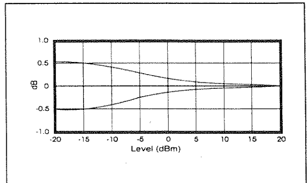
Temperature Influence ( \pm 4 ^{\circ} from calibration)
