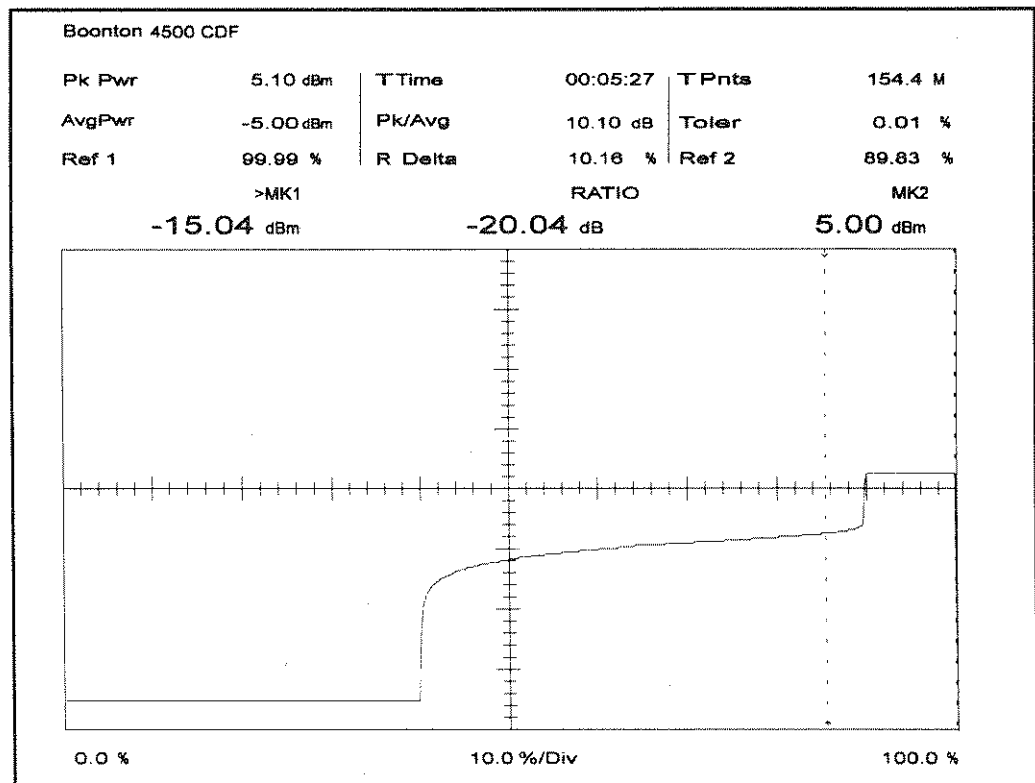
Figure 3-13. CDF Display
