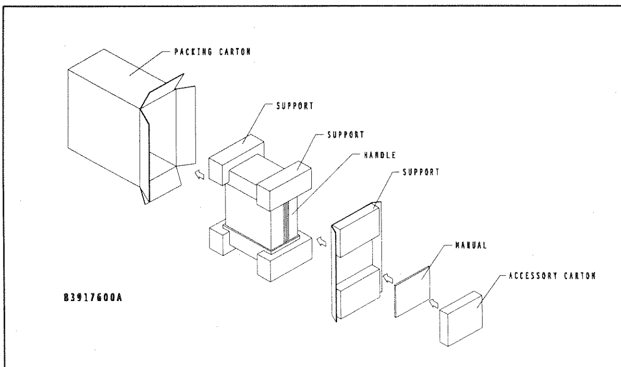
Figure 2-1. Packaging Diagram
