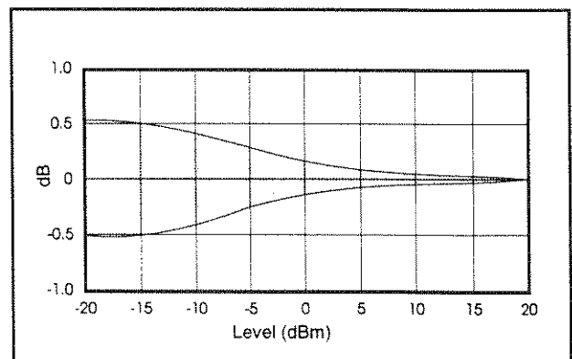
Temperature Influence ( \pm 4^\circ from calibration)
