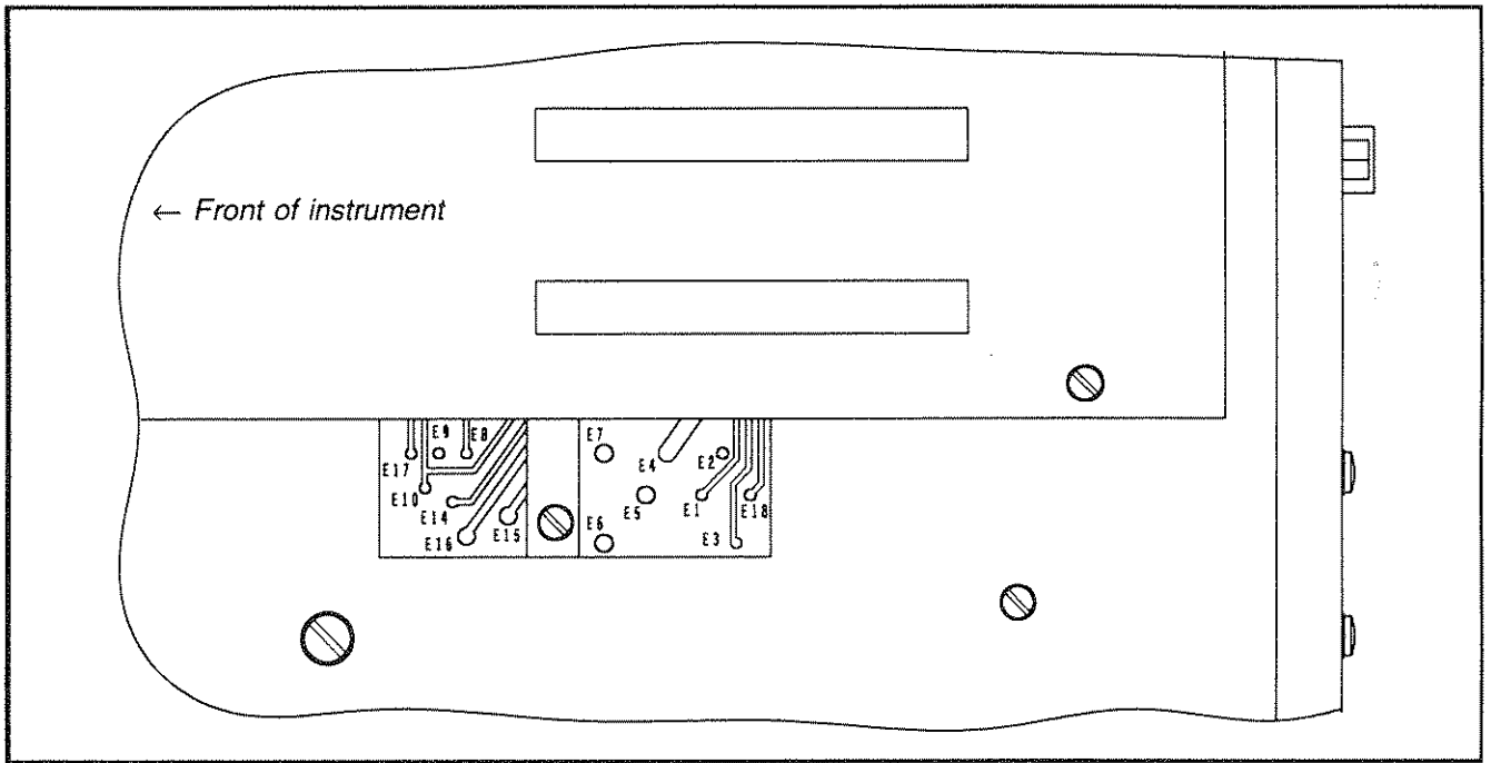
Figure 7-2. Power Supply Test Points
