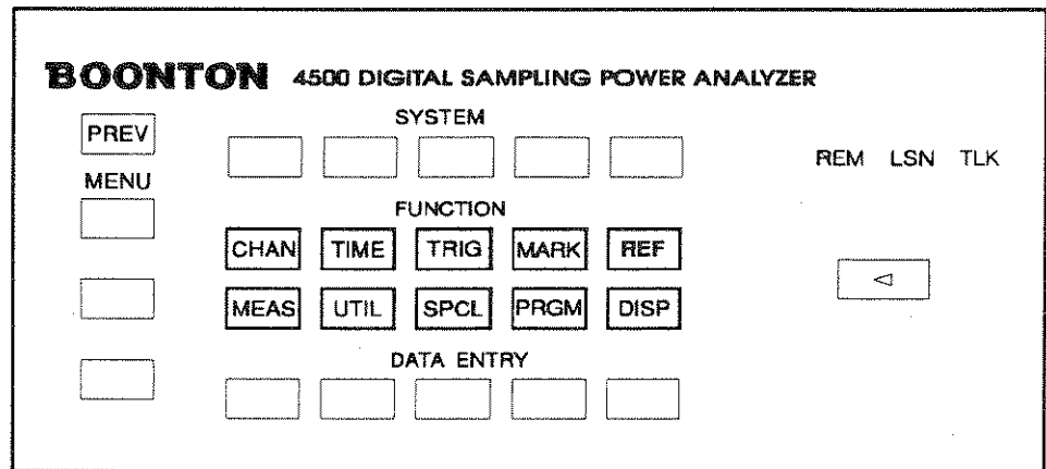
Figure 4-11. Function Keys
