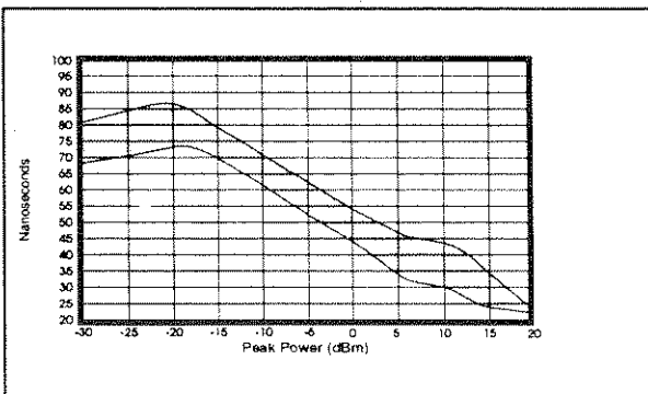
*Typical Risetime in High BW Mode
