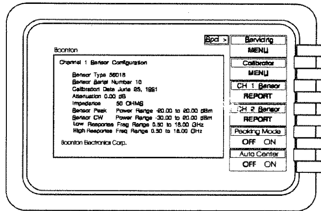
Figure 4-4b. Chan 1 Sensor Configuration Report
